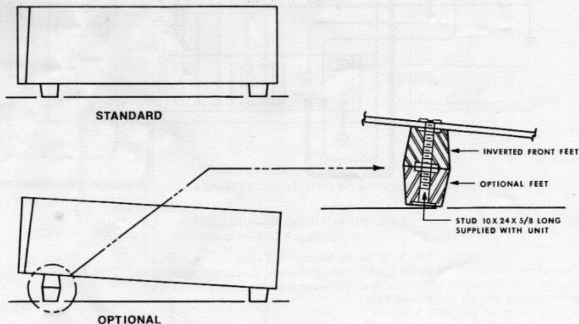
Figure 2-6. Viewing Angle Options
