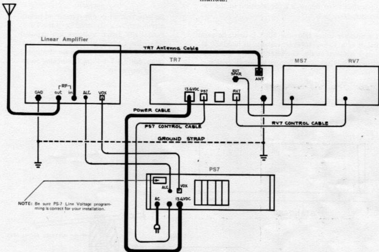
Figure 2-5. Connecting the RV-7 Remote VFO and a Linear Amplifier
