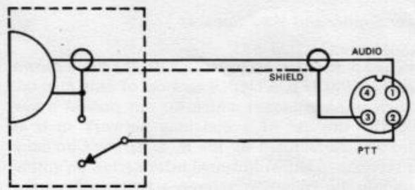
Figure 2-3. TR-7 Microphone Connection
